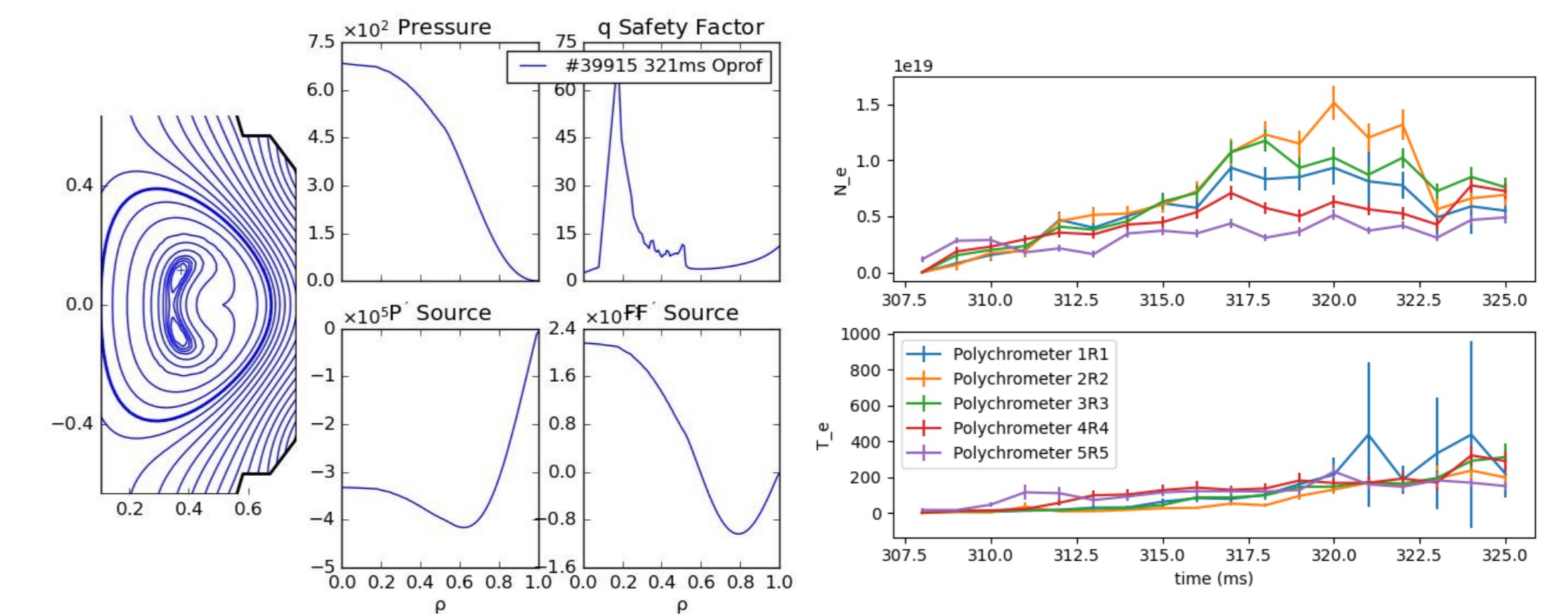
Fig. 9. EFIT result in 321ms
