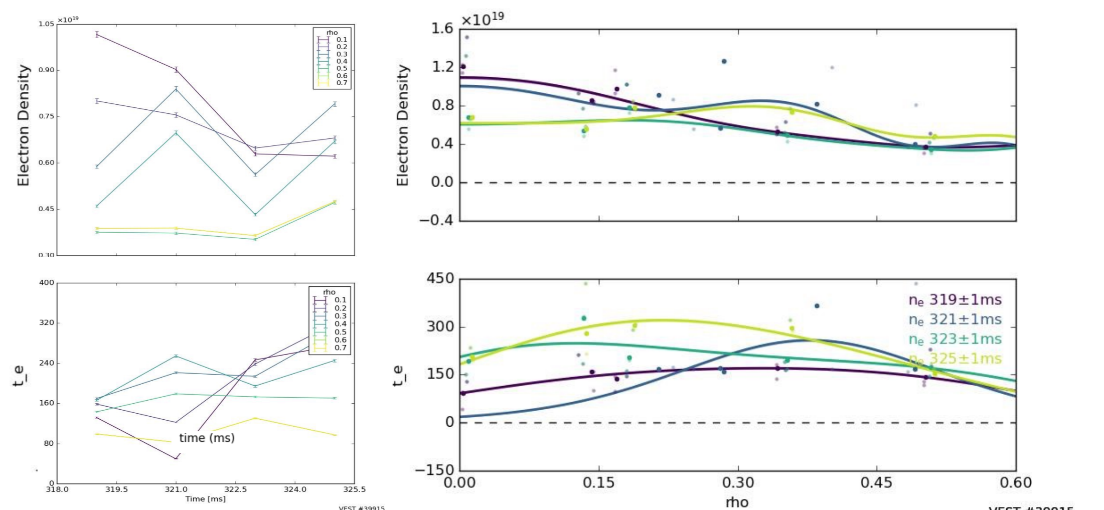
Fig. 11. 1D fit of sliced data for 39915 shot.
