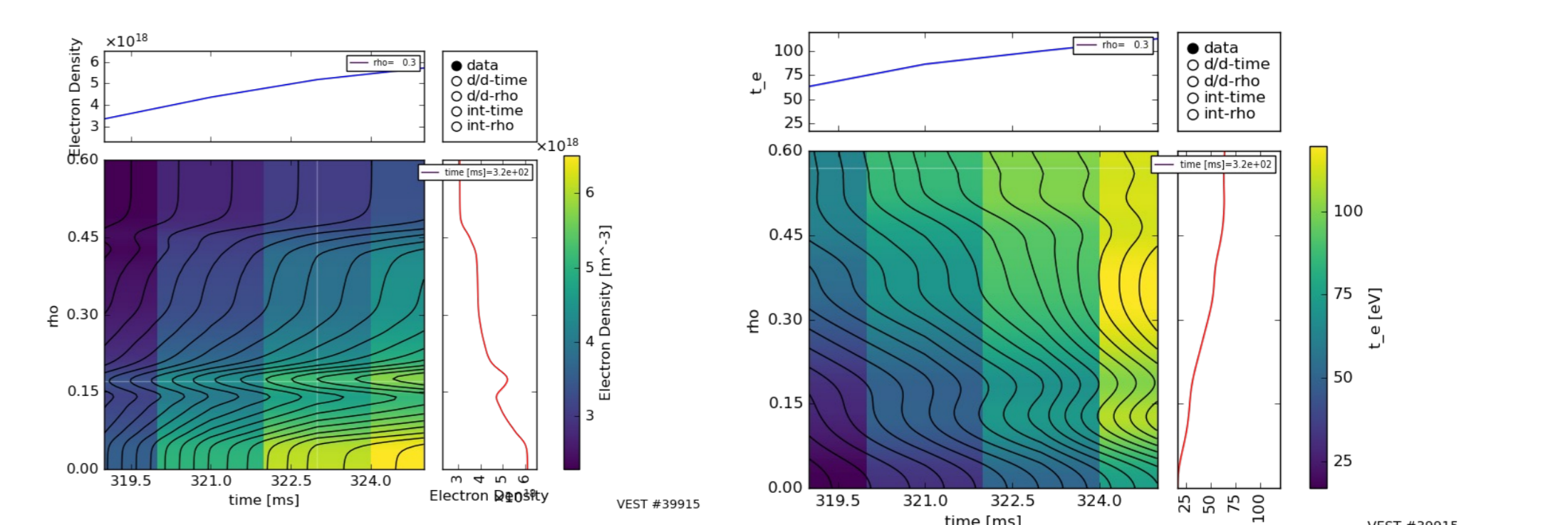
Fig. 12. 2D fit of raw data for 39915 shot.
